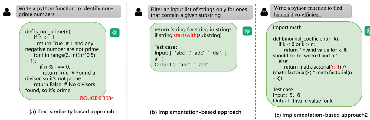
Fig. 1: A motivation example
