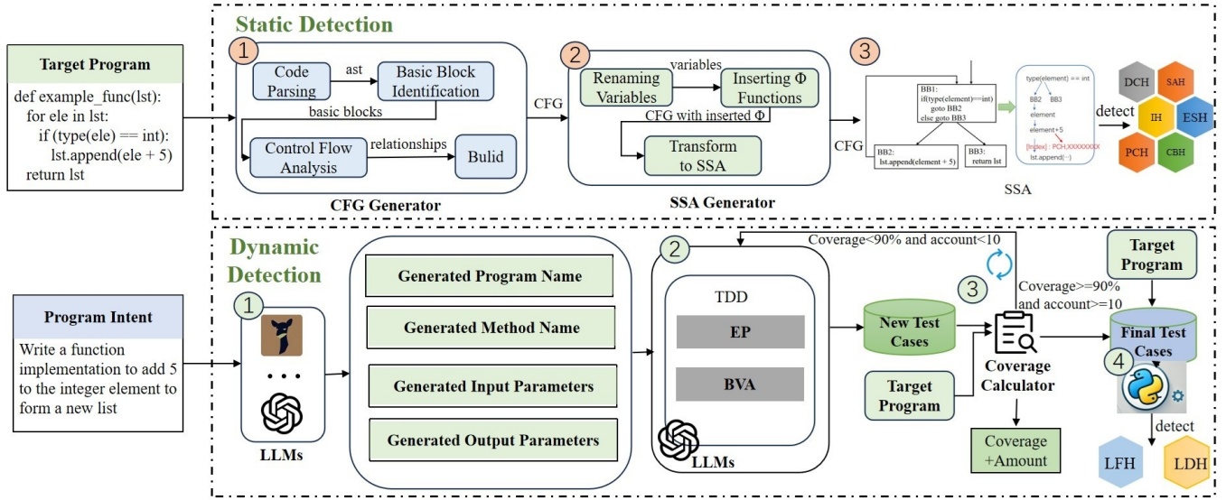
Fig. 2: The hallucination detection framework
