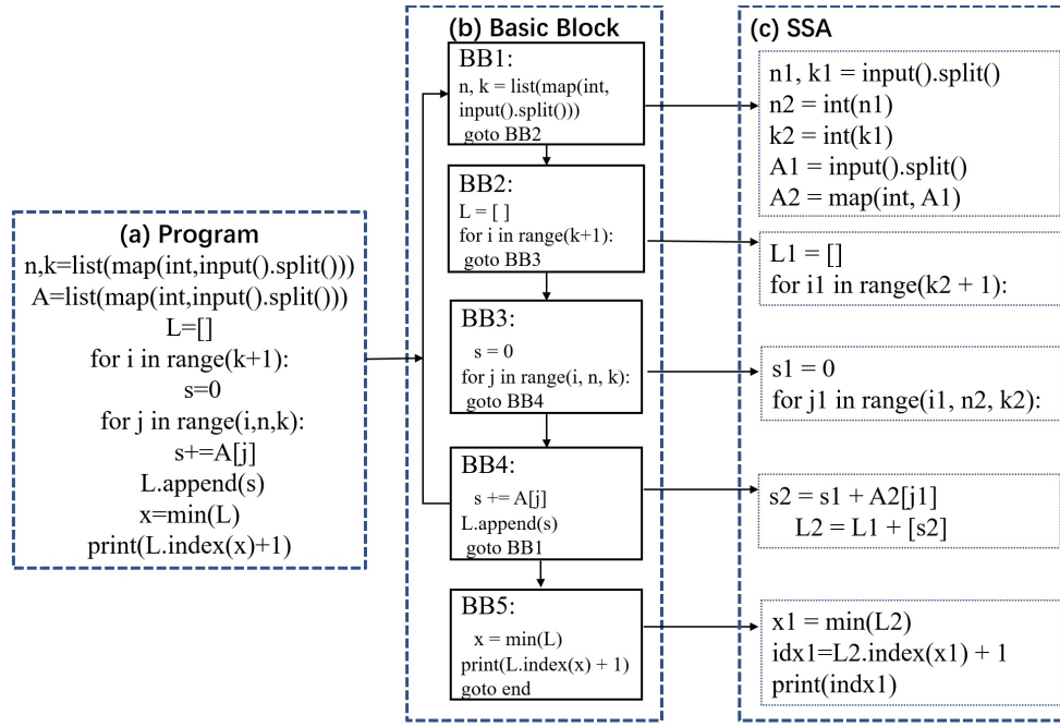
Fig. 3: Constructing the SSA of a program
